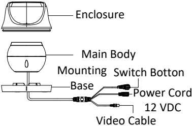
Figure 1-2 Overview of Type II Camera
