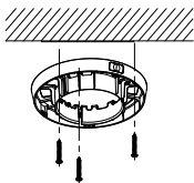
Figure 2-5 Fix the Mounting Base
