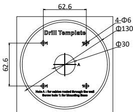
Figure 2-17 Drill Template
